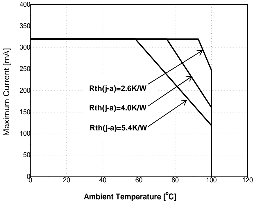
Fig 8. Maximum Forward Current vs. Ambient Temperature, T_j(\text{max.}) = 125^\circ\text{C} , I_F = 0.32\text{A}
